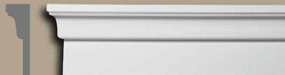
CSH 1035 (See MD 1035 on page 177) • 3" Projection • 9" Height • Matches K 2701
